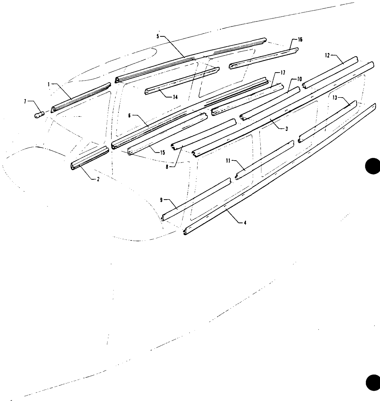
Figure 15B. Window Curtain Installation
