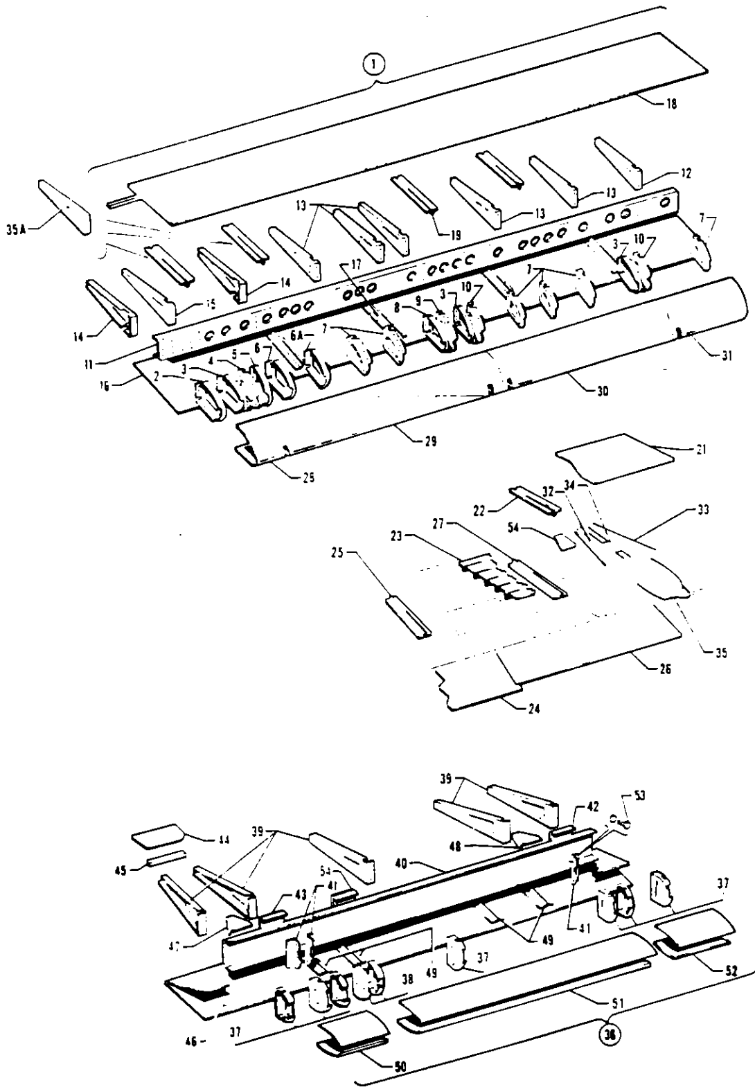
Figure 3. Flap and Aileron Assemblies
