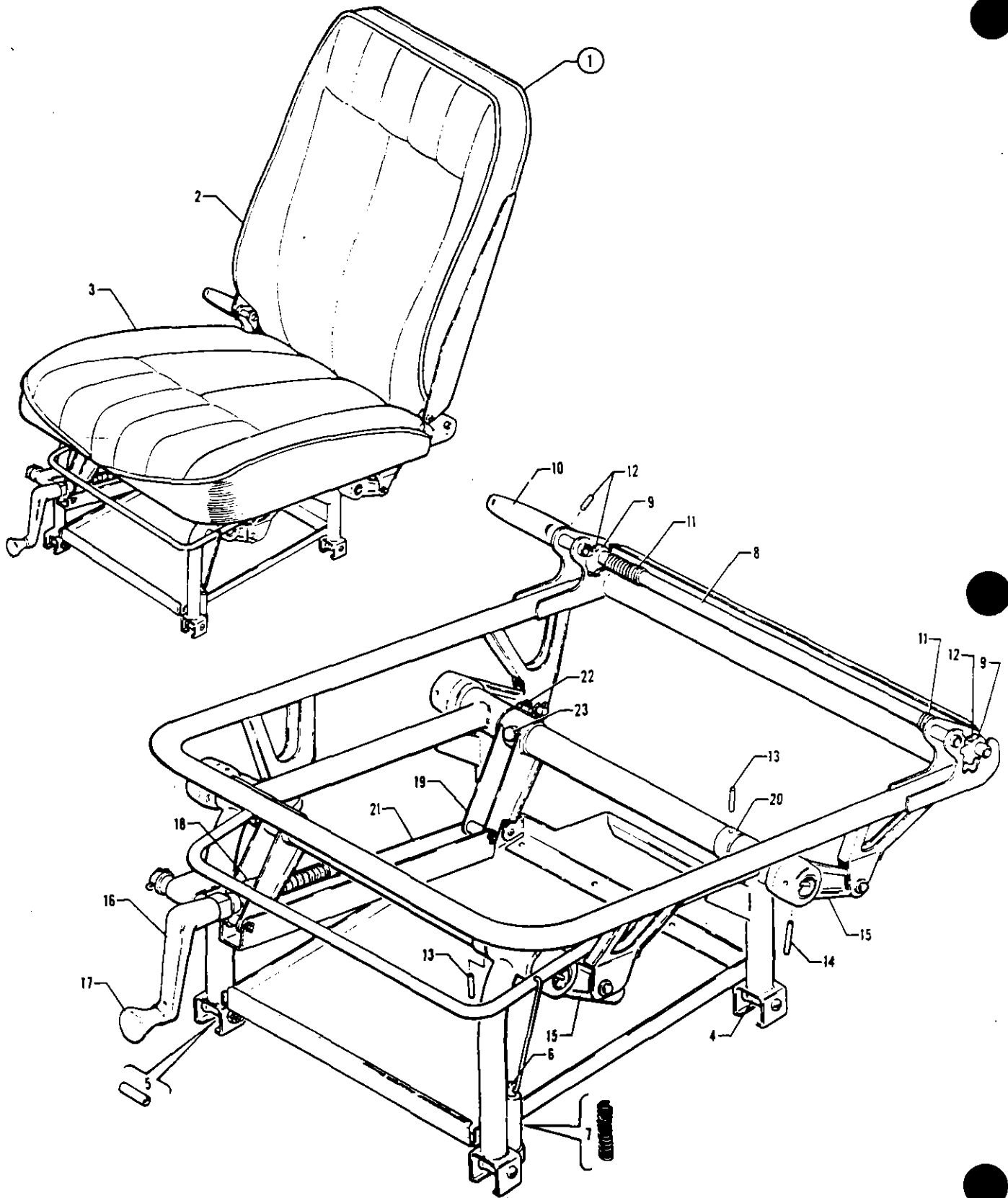
Figure 18B. Vertically Adjustable Seats Installation (PA-30 with Serial Nos. 30-1717, 30-1745 and up) (PA-39 with Serial Nos. 39-1 and up)
