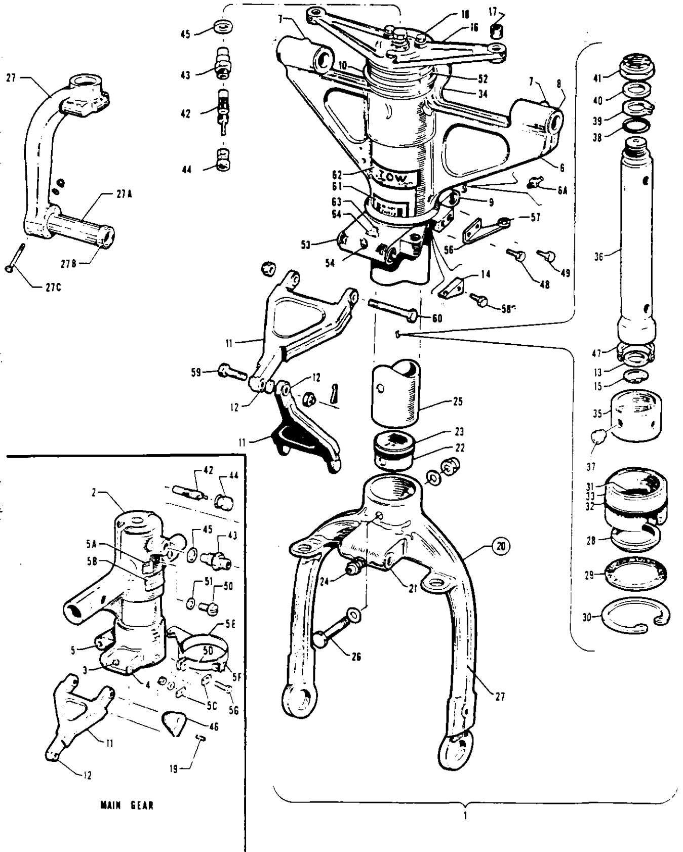
Figure 2c. Landing Gear Strut Assemblies
