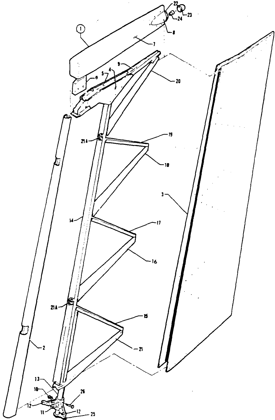
Figure 33. Rudder Assembly
