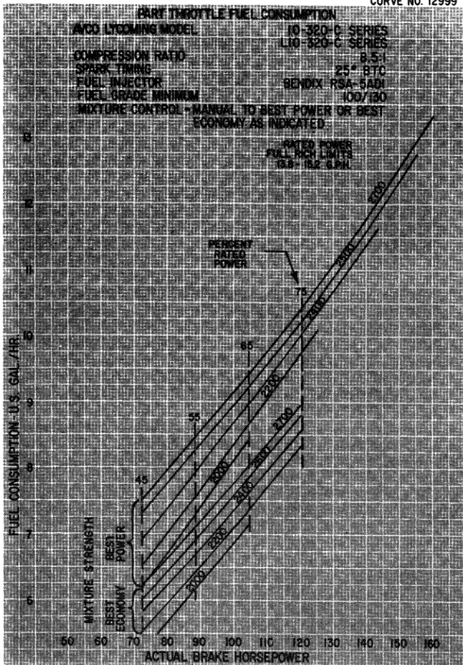
Figure 3-12. Part Throttle Fuel Consumption - IO-320-C, L10-320-C
